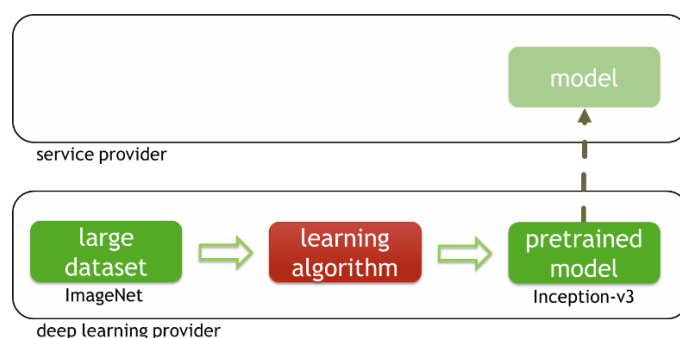
Figure 7: using a pre-trained model.
