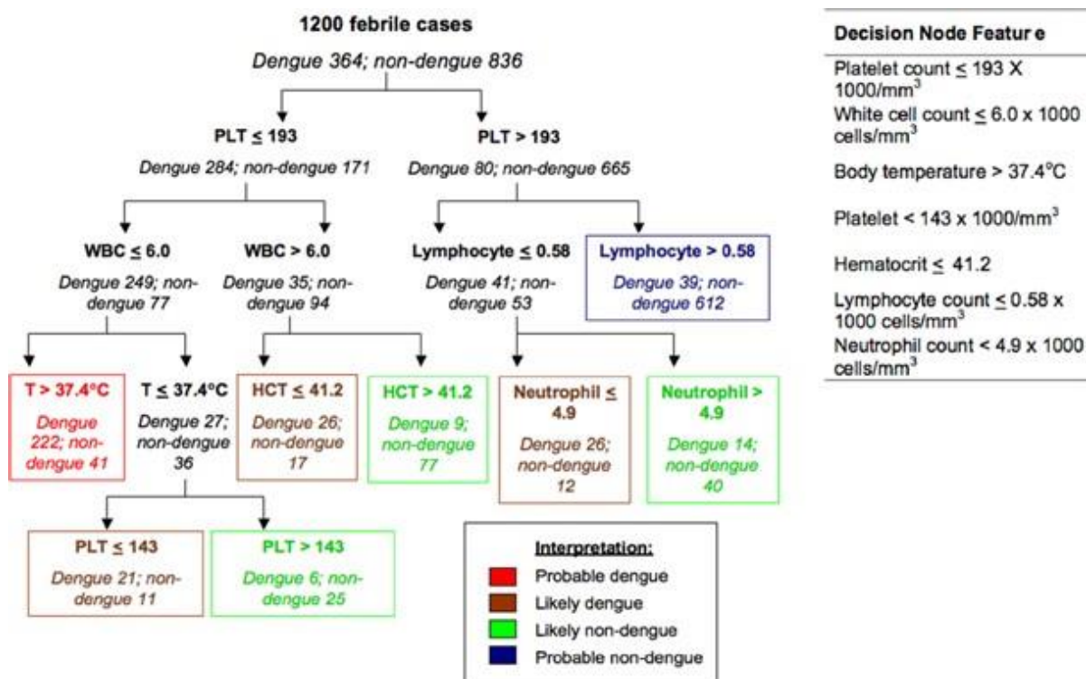
Figure 2: example of a model of categories expressed in the form of logic rules organised in a decision tree 15 .
