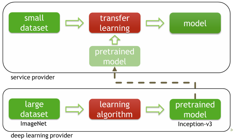
Figure 10: retraining and using a pre-trained neural network by transfer learning.
