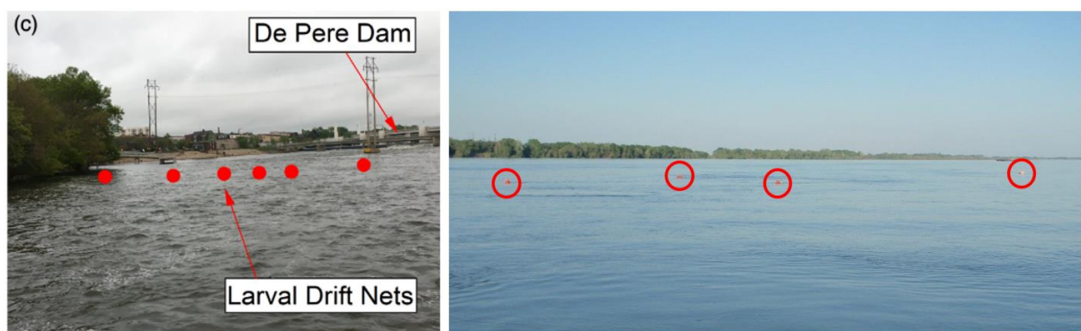
Figure 10: D-nets set perpendicular to the shore (left, adapted after Tucker et al., 2021), or in pairs in the mid-channel (right, © DDNI, M. Paraschiv).
