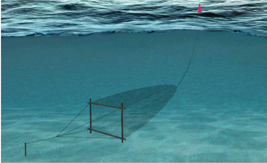
Figure 14: Schematic drawing of a stow net (adapted after He et al. (2021)).
