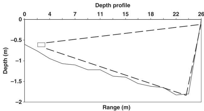
Figure 18: Ideal profile of the river bottom for stationary hydroacoustic surveys. Gradually descending slopes exclude areas with acoustic shadows where detections are impossible to realize (adapted after Auer & Baker (2007)).
