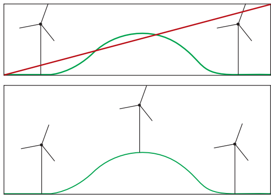
Figure 2. Example of wind turbines close to and at a high point; the scale of the landscape must be preserved
