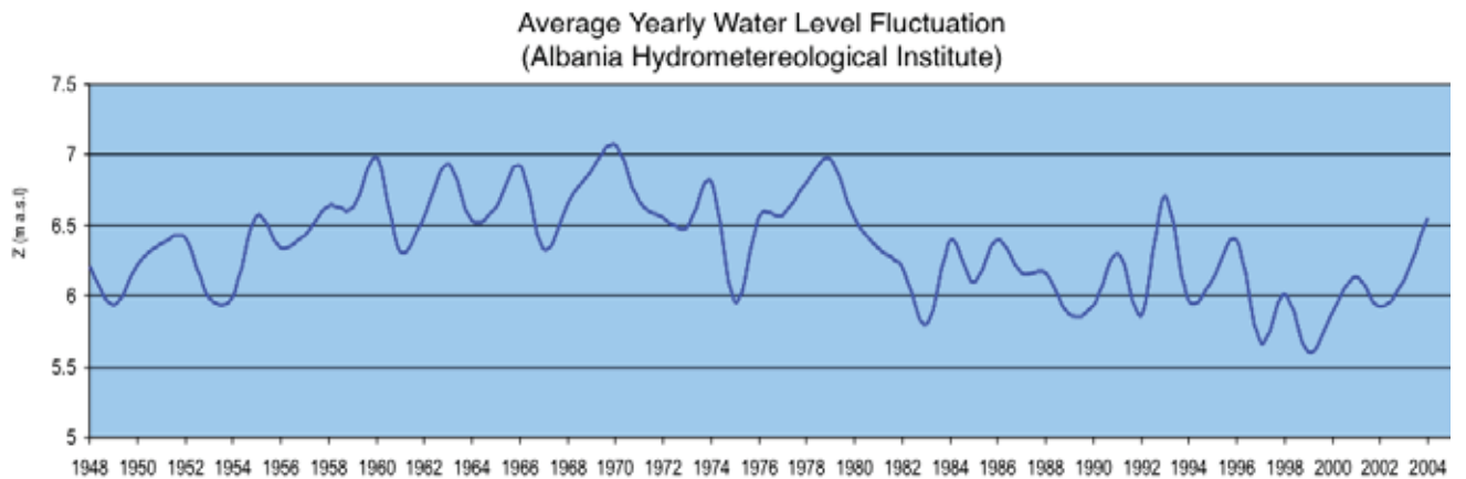
Figure 18. Average yearly fluctuation (meters above sea level) for Skadar/Shkodra Lake from 1950 to 2004 (Albania Hydrometeorological Institute)
