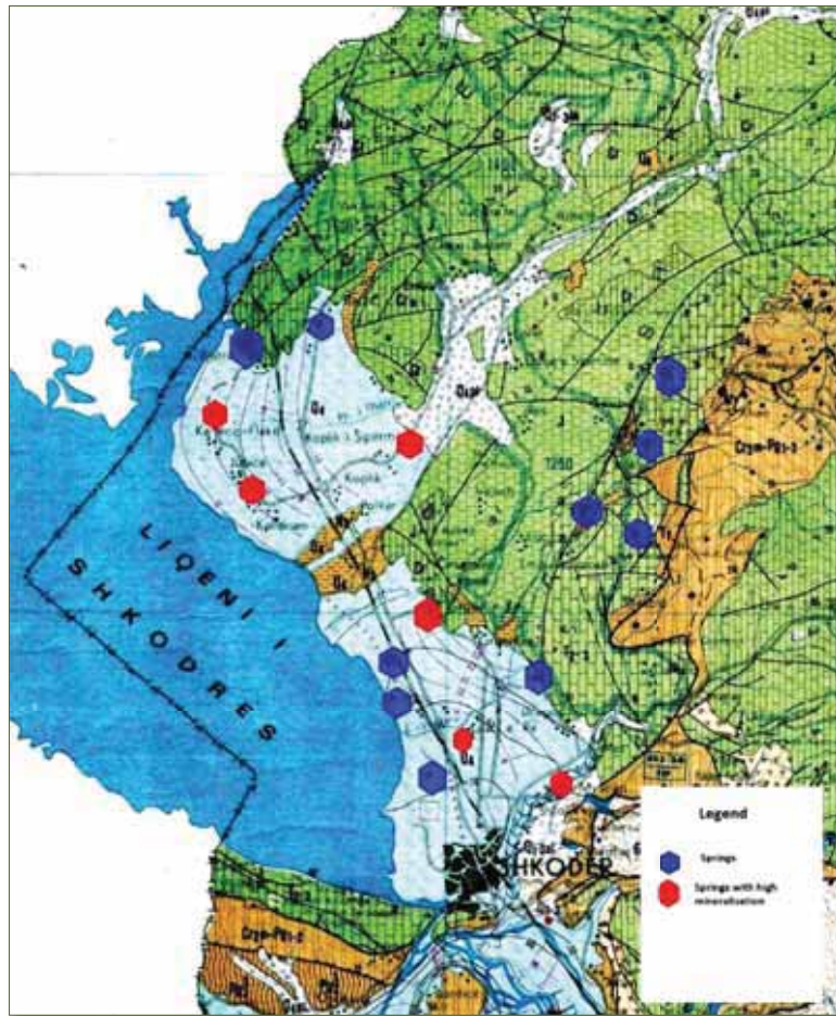
Figure 16. The springs and wells in the Albanian section of Skadar/Shkodra Lake (Hydrogeological Map of Albania 1:200,000, Albanian Geological Service)
