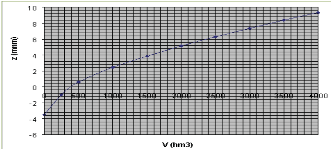
Figure 13. The total volume of Skadar/Shkodra Lake (x-axis) varies depending on the water level (y-axis, in metres above sea level) (Water Basis of Montenegro 2001)
