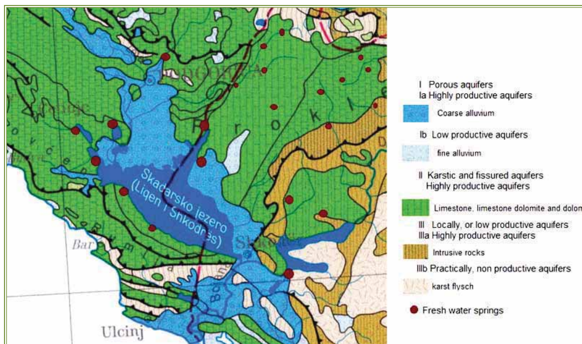
Figure 12. Simplified hydrogeological map of the Skadar/Shkodra Lake and Buna/Bojana River area (adapted from Eftimi R. 2010)
