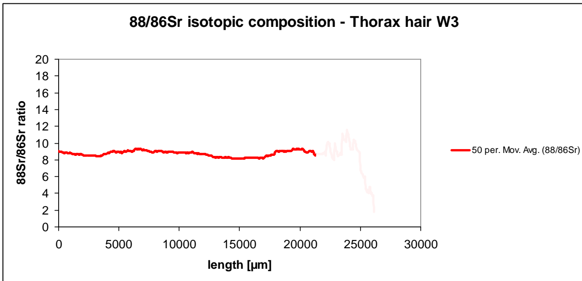
Figure 14: 88/86 Sr isotopic ratio along thorax hair W3. (The ratio is a raw estimate and not analyzed in isotope ratio mode).
