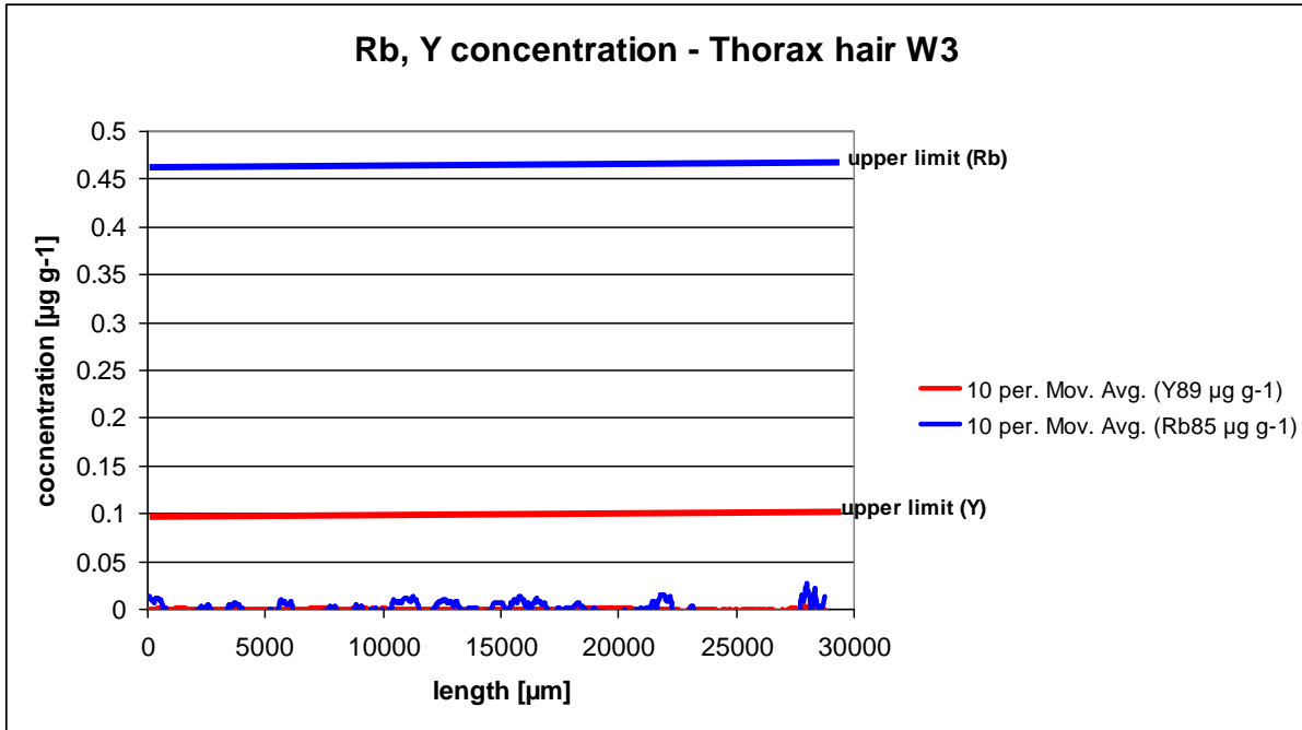
Figure 15: Rb and Y concentration along thorax hair W3. (Upper limits correspond to published elemental ranges)
