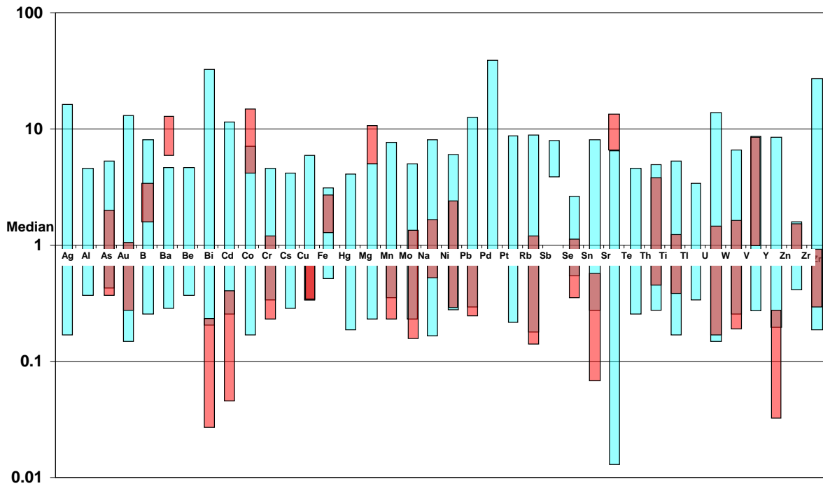
Figure 4: Comparison of the thorax hair (red) range (given by the average +/- SU) and the “normal range” published in literature. 8 The values are set relative to the median of the “normal range”.
