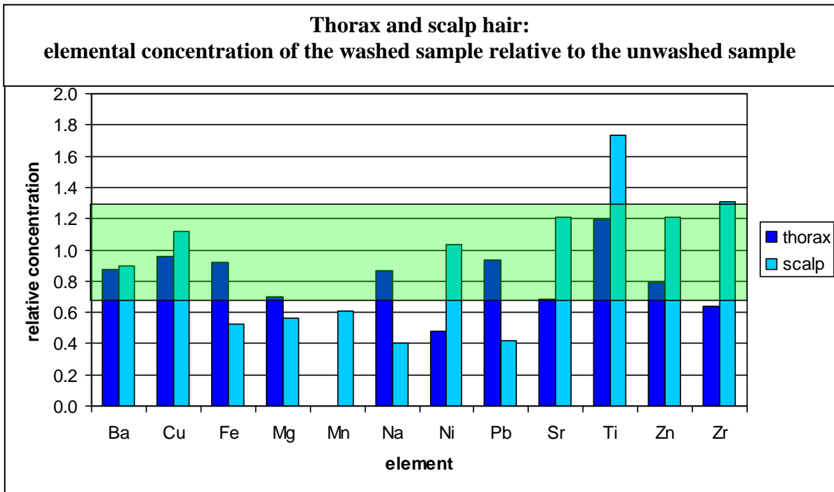
Figure 2: Relative elemental concentration of the washed hair relative to the unwashed hair for thorax and scalp hair of the person concerned.
